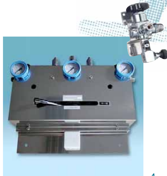
DECOMPRESSION UNITS FOR CORROSIVE GAS Material stainless steel AISI 316 L REGULATORS FOR NH 3 AMMONIA Material aluminium, internal parts 316 L Working pressure 30 bar to 200 bar
